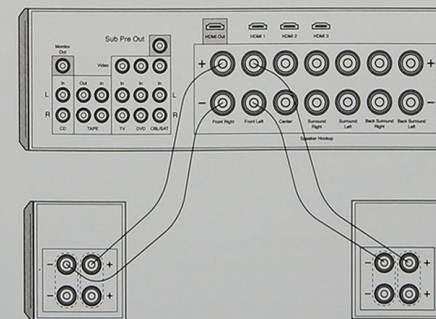
Figure 5 Standard Connections
