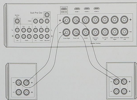
Figure 5 Raccordements standard
