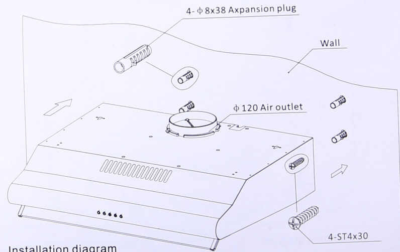
Installation diagram
